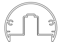
SERIES 300W (SERIES 300W IS DESIGNED TO BE WELDED TO THE POST)
