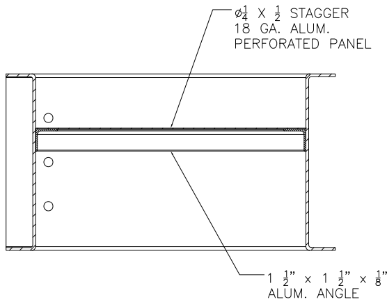
TYPICAL CROSS SECTION A-A
