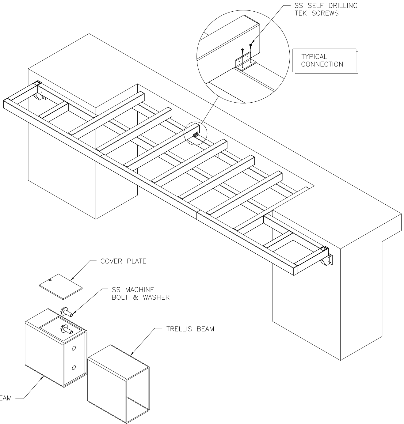
SPLICE DETAIL
