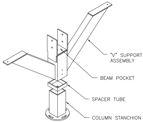
— SUPPORT ARM DETAIL
